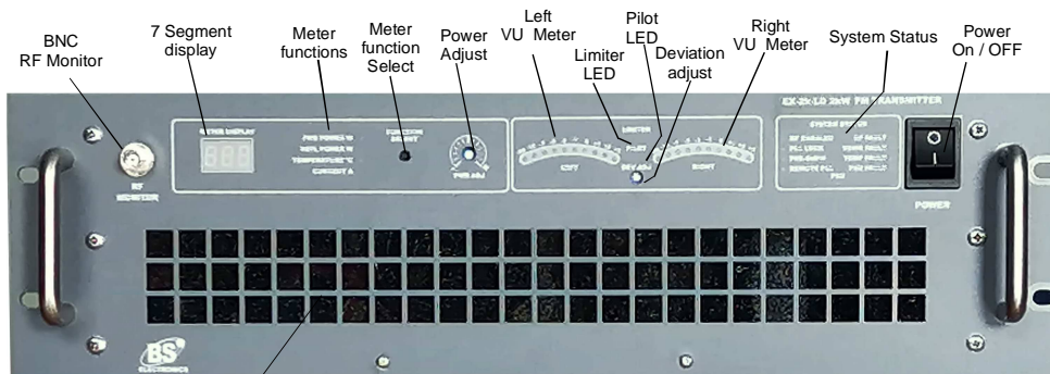
EX-2K-LD 2kW FM TRANSMITTER FRONT PANEL
